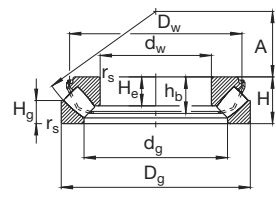
293E, 294E d_w \geq 220 mm
