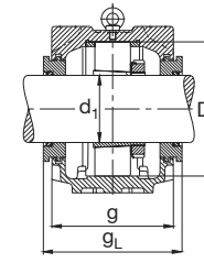
Anel labirinto TSV
