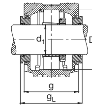
Anel labirinto TSV
